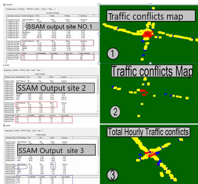
Figure 3. Summary of the SSAM software for study areas.
